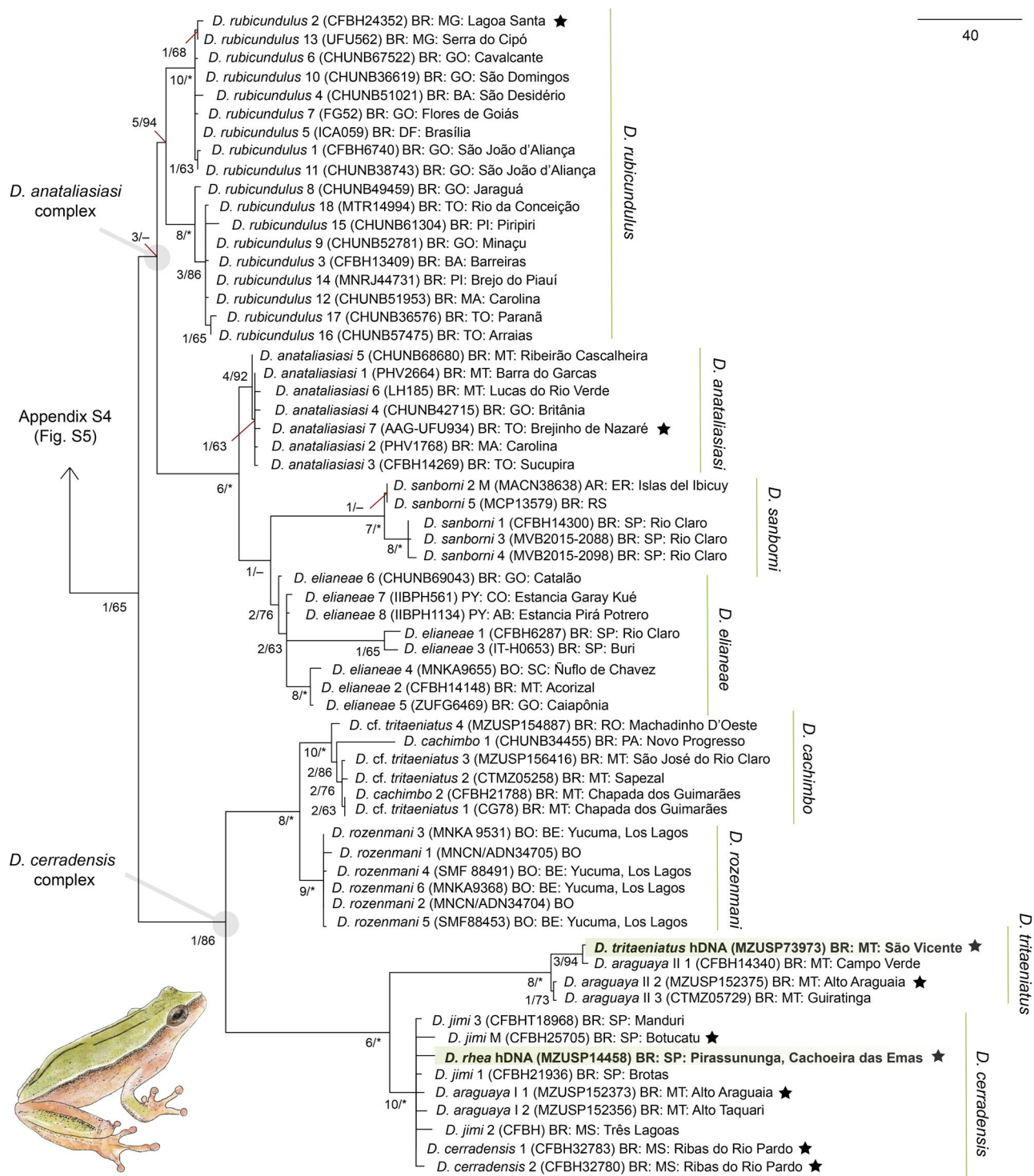
Fig. 1. Phylogenetic relationships of the Dendropsophus rubicundulus clade. Strict consensus tree recovered in the final round of outgroup expansion (13,653 steps). Numbers around nodes are Goodman-Bremer support/jackknife absolute frequencies. Asterisks indicate 100% jackknife values; < 50% values are omitted. Black stars indicate topotypic samples. Names next to green bars indicate the newly revised taxonomy. See the complete topology for MP and ML analyses in Appendix S4: Figs. S5 and S6, respectively. Abbreviations: AR – Argentina (provinces: ER – Entre Ríos); BO – Bolivia (departments: BE – Beni, SC – Santa Cruz); BR – Brazil (federative units: BA – Bahia, DF – Distrito Federal); GO – Goiás; MA – Maranhão; MS – Mato Grosso do Sul; MT – Mato Grosso; PA – Pará; PI – Piauí; RO – Rondônia; RS – Rio Grande do Sul; SP – São Paulo; TO – Tocantins; PY – Paraguay (departments: AB – Amambay, CO – Concepción).
